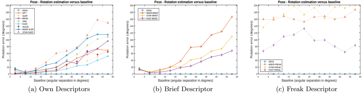
Figure 6: Mean estimation error of relative stereo camera rotation over varied camera baselines 4 .
