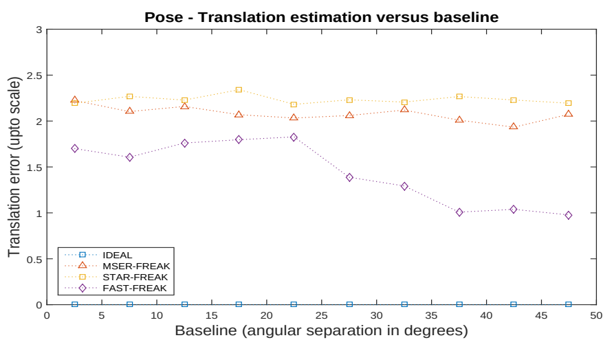
Figure 4.18: Translation error of stereo camera over varied camera baselines.
