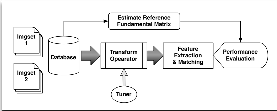
Figure 4.2: Evaluation Pipeline
