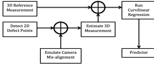
Fig. 4. Simulation procedure.
