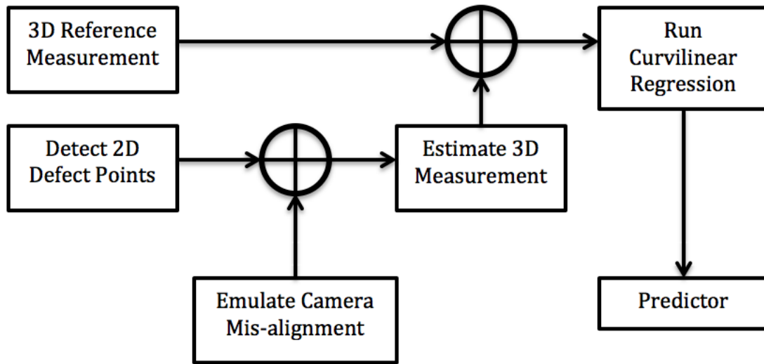
Figure 3.2: Simulation procedure.
