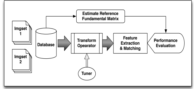
Figure 2: Evaluation Pipeline
