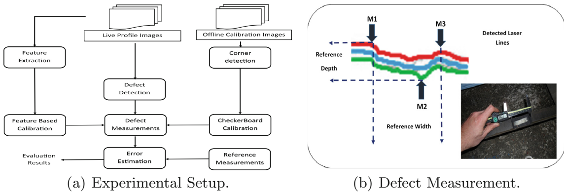
Fig. 3. Evaluation scenario
