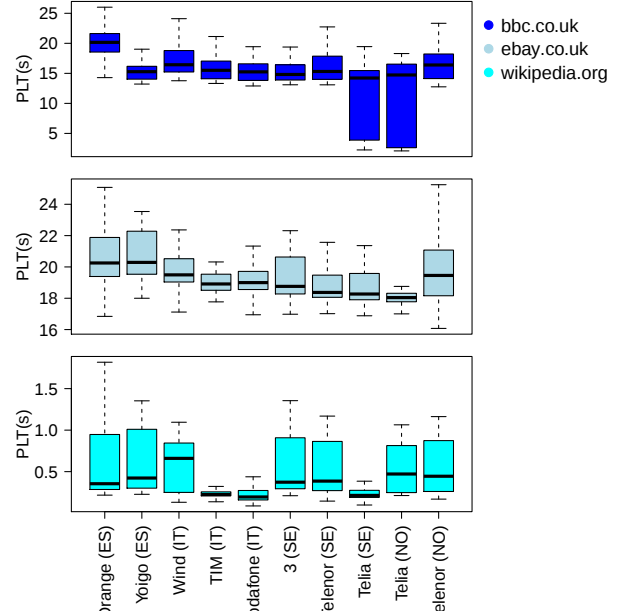
Figure 3: Differences in PLT of target web pages across 10 commercial operators.
