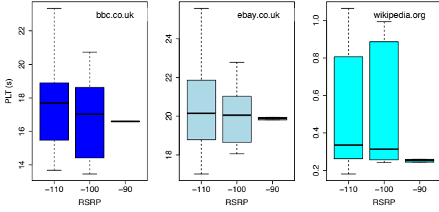
Figure 4: PLT at different signal quality levels for a particular MONROE node.
