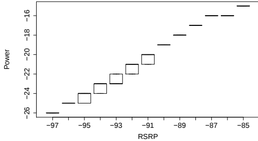
Figure 6: RSRP at different power levels
