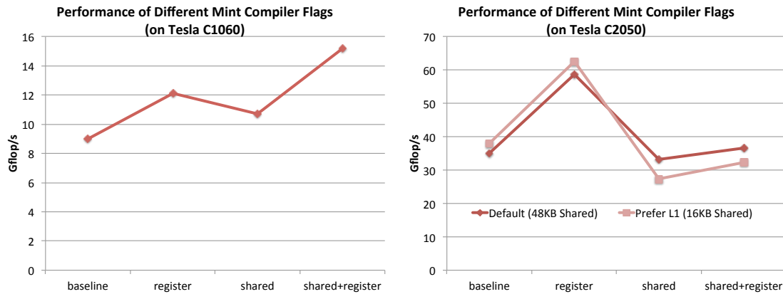
Figure 7.5: On the C1060 (left), the best performance is achieved when both the shared memory and register flags are used. The results are with the nest(all) , tile(32,4,1) and chunksize(1,1,1) clause configurations. The shared flag is set to 8. On the C2050 (right), the best performance is achieved when a larger L1 cache and registers are used. The results are with the nest(all) , tile(64,2,1) and chunksize(1,1,1) configurations. The shared flag is set to 8.
