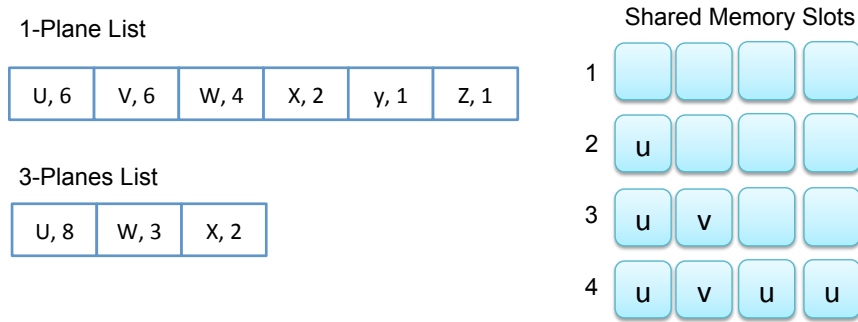
Figure 5.8: Filling shared memory slots with selected variables
