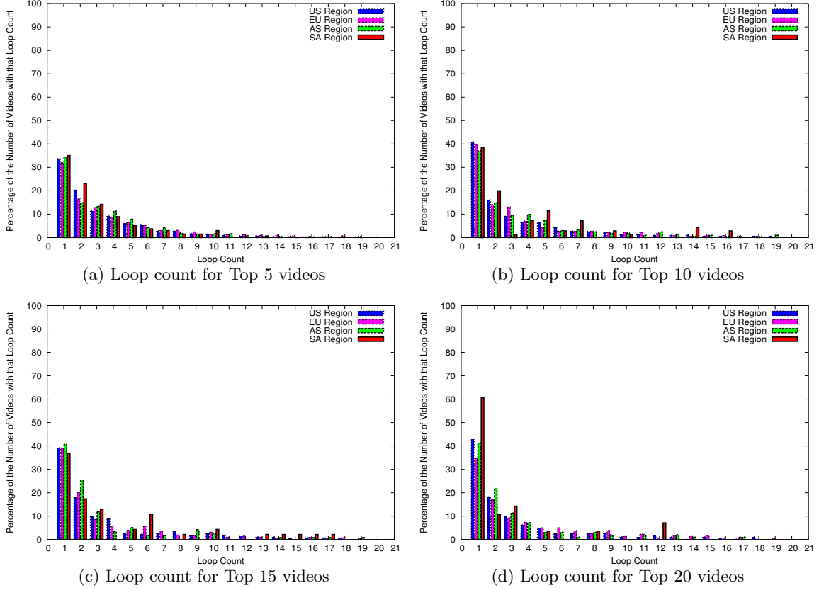
Figure 6: PlanetLab-based loop count measurement for random selection from related list
