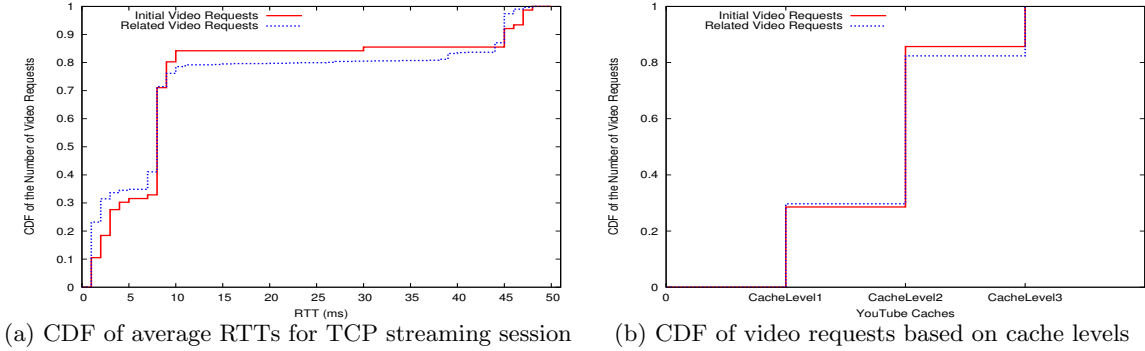
Figure 7: Distribution of video delivery based on response times and cache levels.
