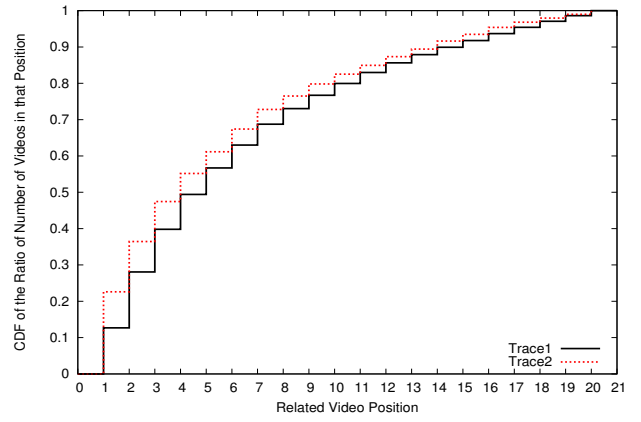
Figure 3: Position of video selected by users from related video list for traces T1 and T2.
