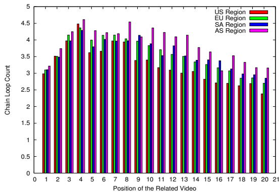
Figure 5: PlanetLab-based loop count measurement for fixed position selection from related list
