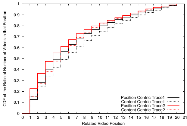
Figure 10: Position of video selected from related video list after reordering.
