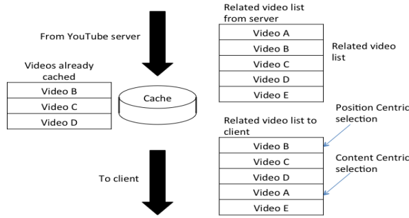
Figure 9: Reordering of the related video list by the cache
