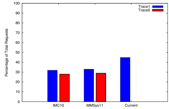
Figure 2: Percentage of videos selected from related video list as reported in earlier studies (IMC10 [19], MMSys11 [17] ) and obtained from an analysis of the trace used in this paper.
