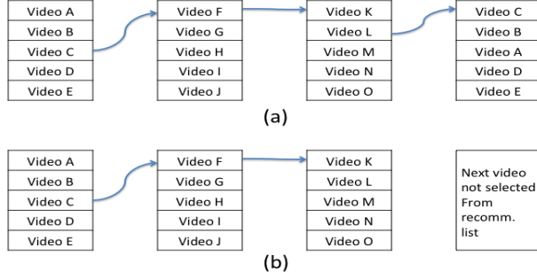
Figure 4: Chain and Loop count example. (a) Example for a loop of length 2, (b) Example of a chain with length 2.
