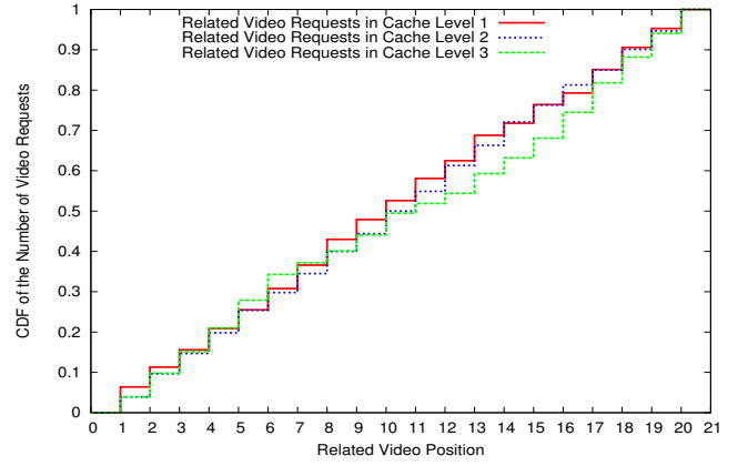
Figure 8: Distribution of position of video in related list compared to all requests originating from the related list.
