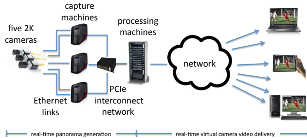
Figure 2: Setup.
