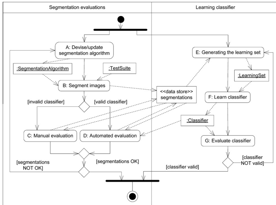
Fig. 3. Image Segmentation Automated Oracle (ISAO).
